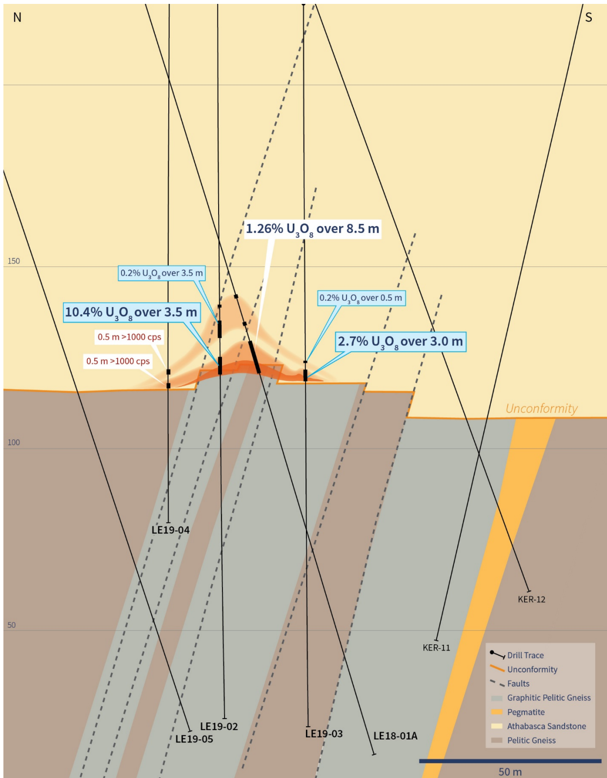
Figure 2 –Cross-Section 4560E
